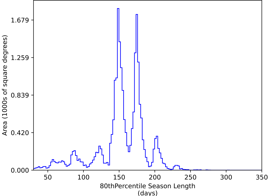
too_elab_heavy_r32_d3_griz_v3.4_10yrs All sky y band: 80thPercentile Season Length
