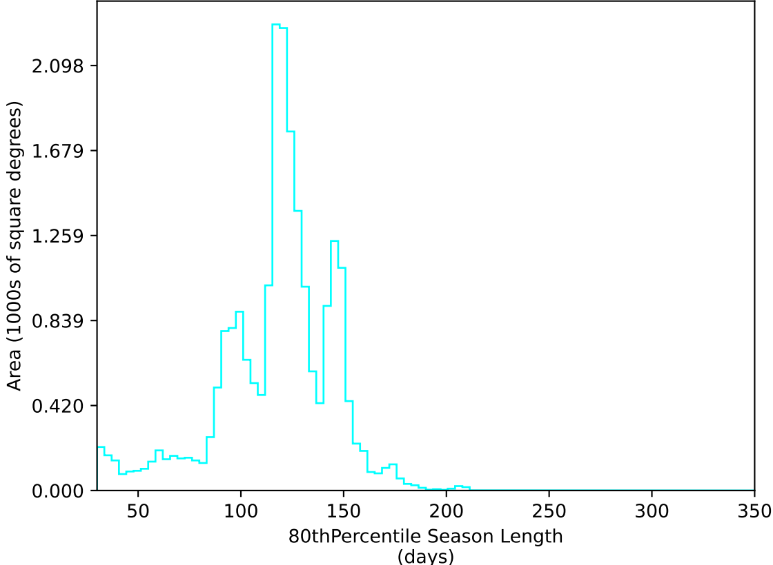
too_elab_heavy_r32_d3_griz_v3.4_10yrs All sky u band: 80thPercentile Season Length
