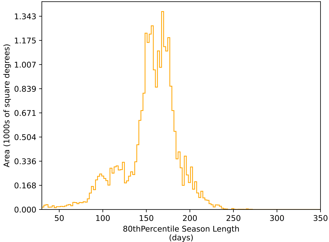
too_elab_heavy_r32_d3_griz_v3.4_10yrs All sky r band: 80thPercentile Season Length
