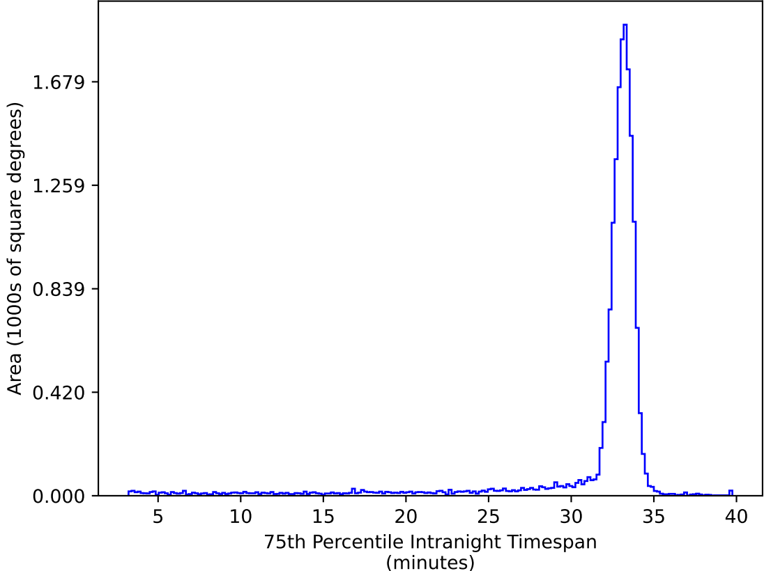
too_elab_heavy_r32_d3_griz_v3.4_10yrs WFD ug bands: 75th Percentile Intranight Timespan
