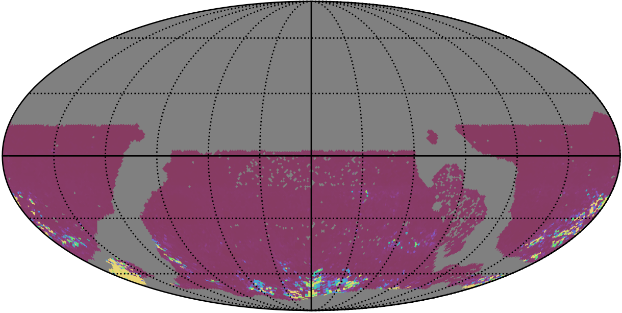
too_elab_heavy_r32_d3_griz_v3.4_10yrs WFD ri bands: 75th Percentile Intranight Timespan
