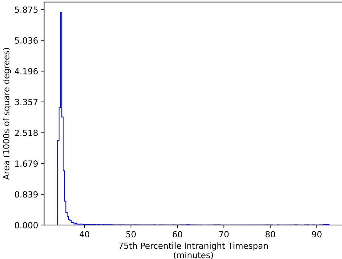
too_elab_heavy_r32_d3_griz_v3.4_10yrs WFD ri bands: 75th Percentile Intranight Timespan
