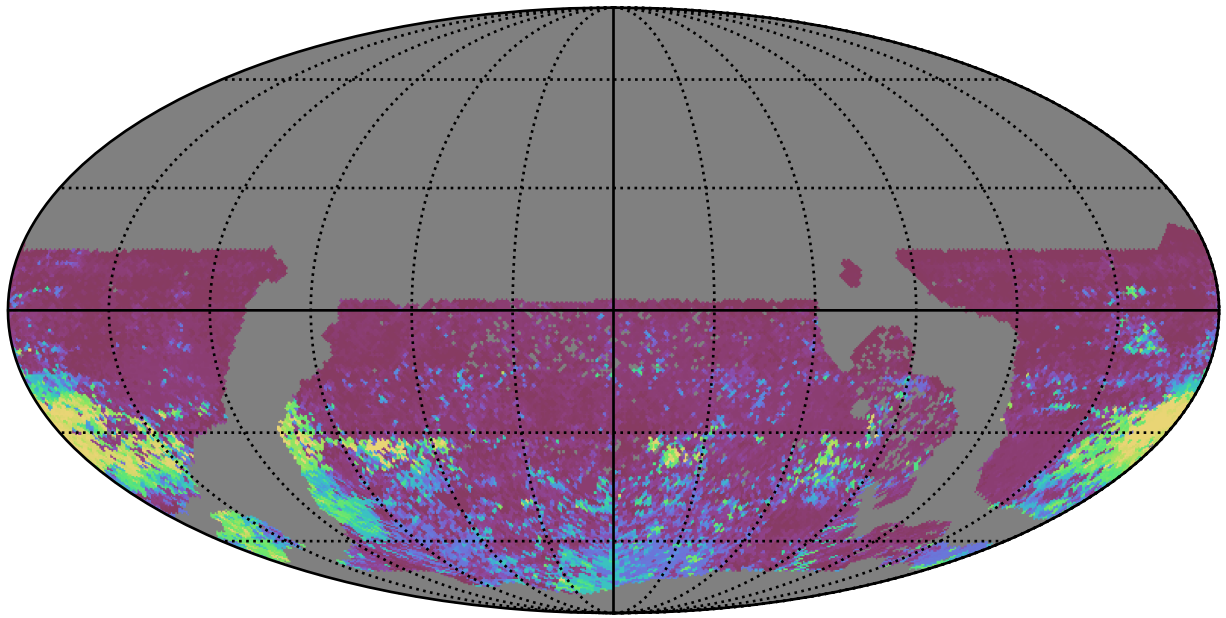
too_elab_heavy_r32_d3_griz_v3.4_10yrs WFD r band: 75th Percentile Intranight Timespan
