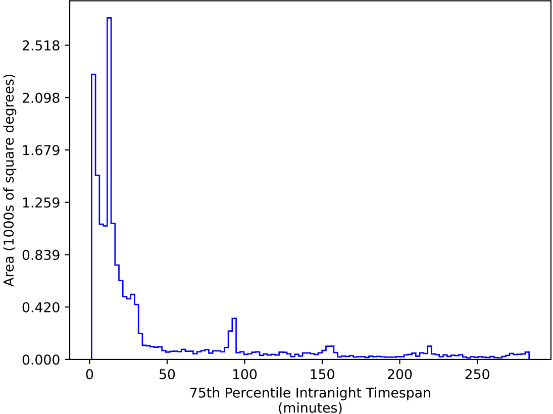
too_elab_heavy_r32_d3_griz_v3.4_10yrs WFD r band: 75th Percentile Intranight Timespan
