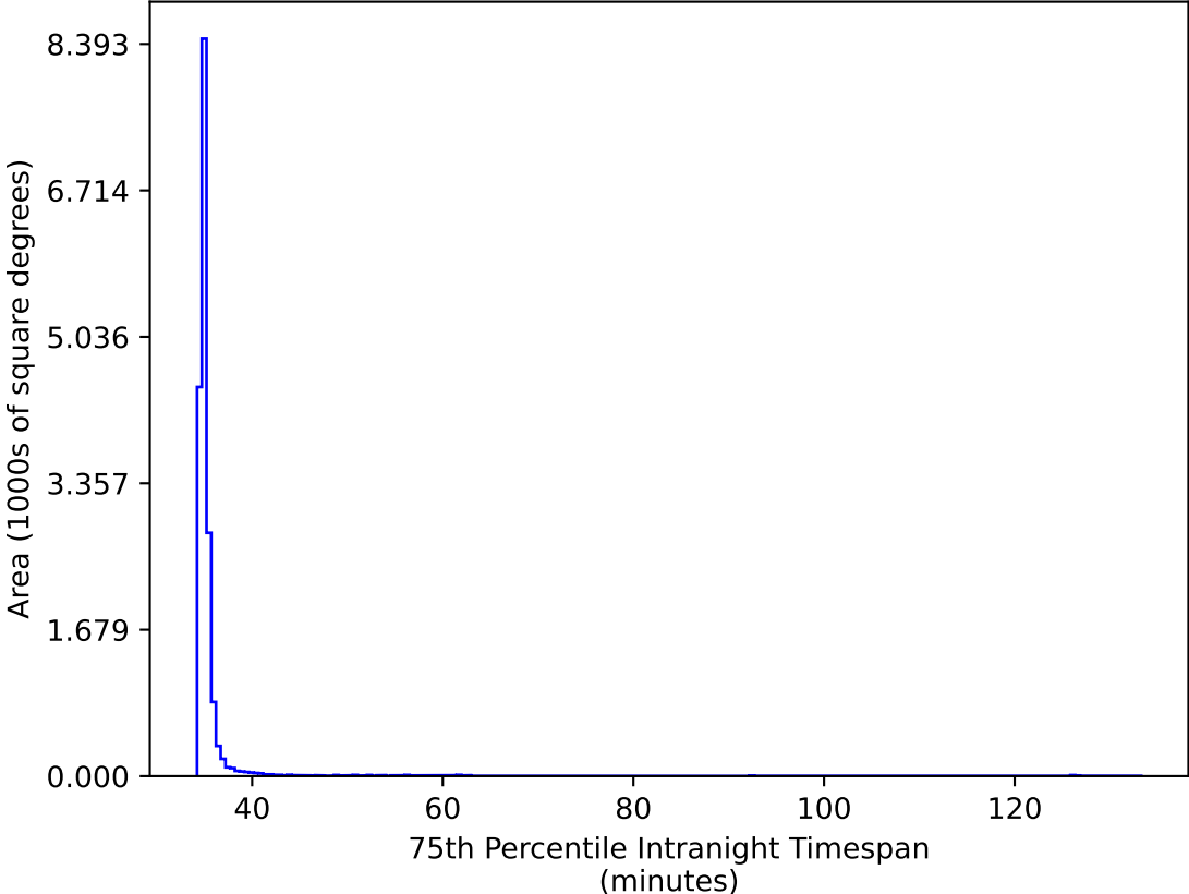
too_elab_heavy_r32_d3_griz_v3.4_10yrs WFD gr bands: 75th Percentile Intranight Timespan
