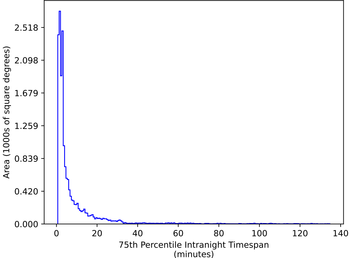
too_elab_heavy_r32_d3_griz_v3.4_10yrs WFD g band: 75th Percentile Intranight Timespan
