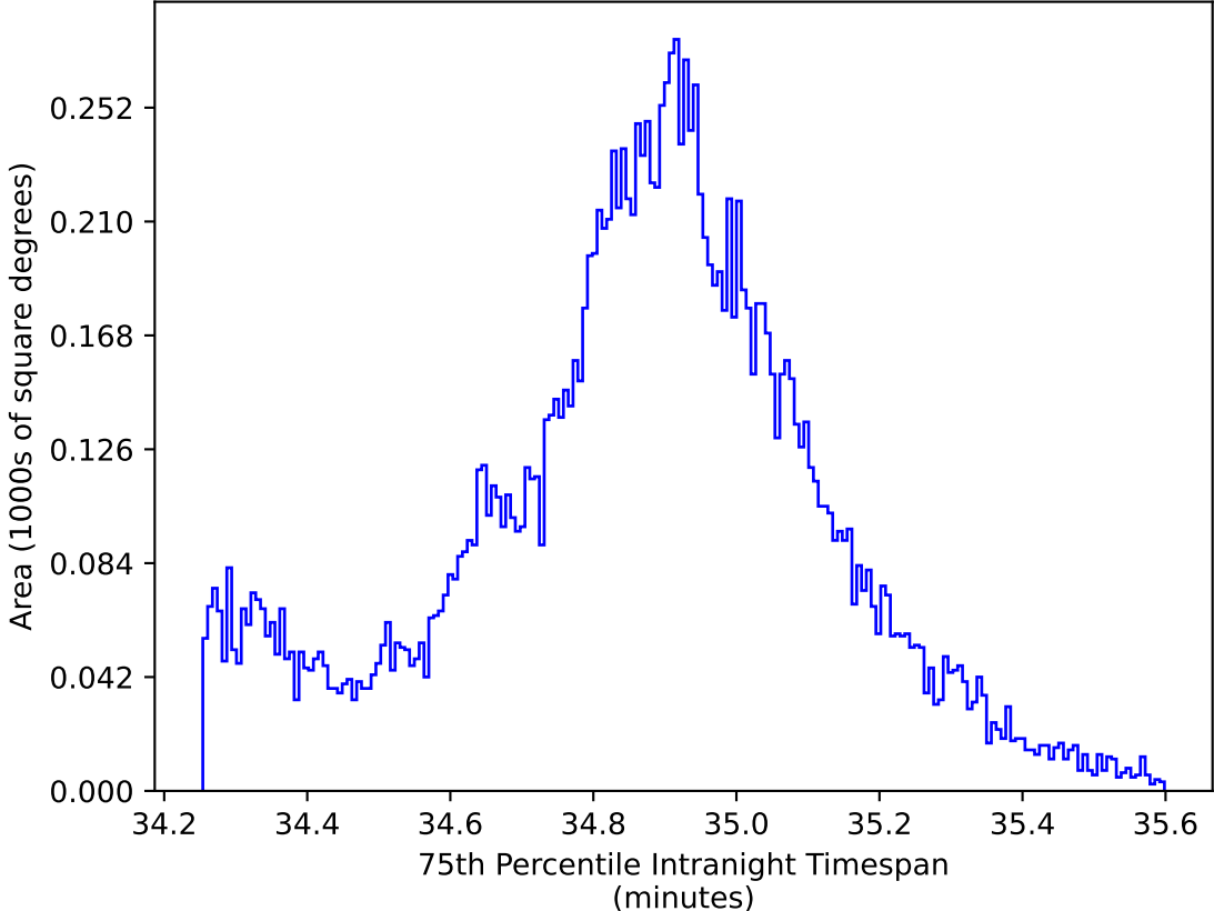
too_elab_heavy_r32_d3_griz_v3.4_10yrs WFD all bands: 75th Percentile Intranight Timespan
