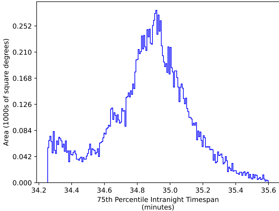
too_elab_heavy_r32_d3_griz_v3.4_10yrs WFD: 75th Percentile Intranight Timespan
