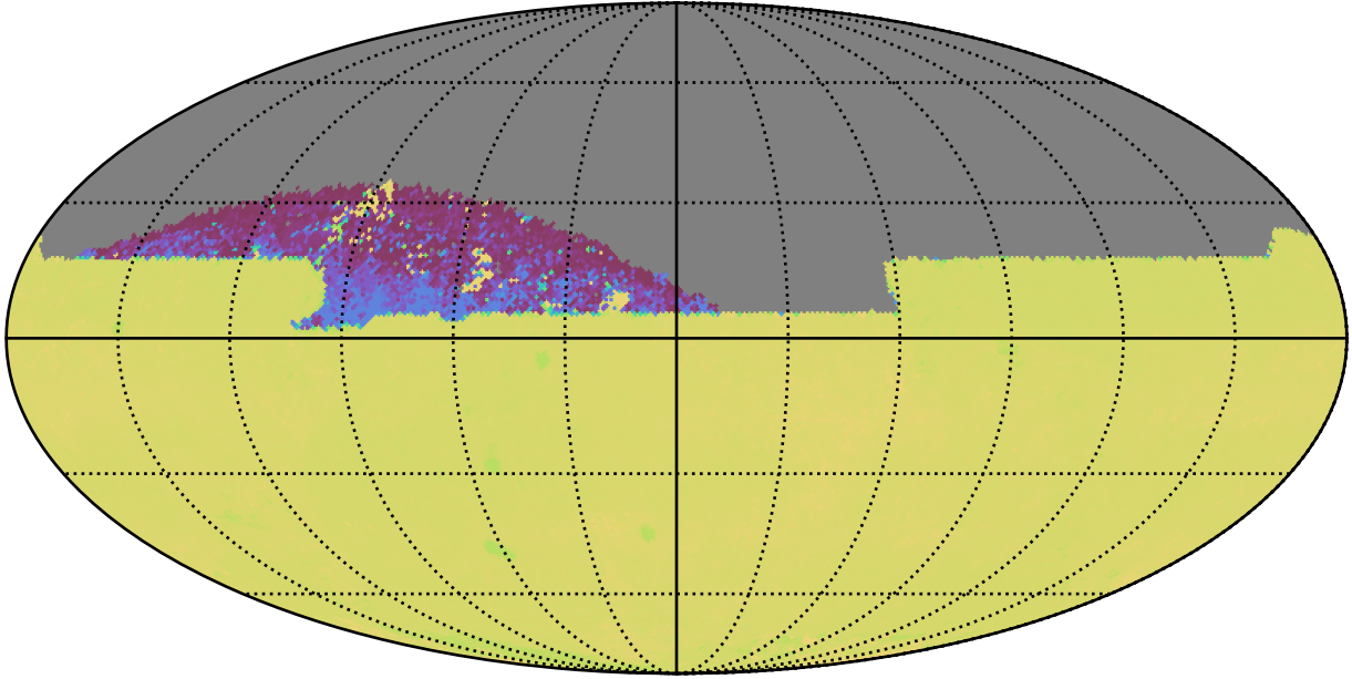
too_elab_heavy_r32_d3_griz_v3.4_10yrs All sky zy bands: 75th Percentile Intranight Timespan
