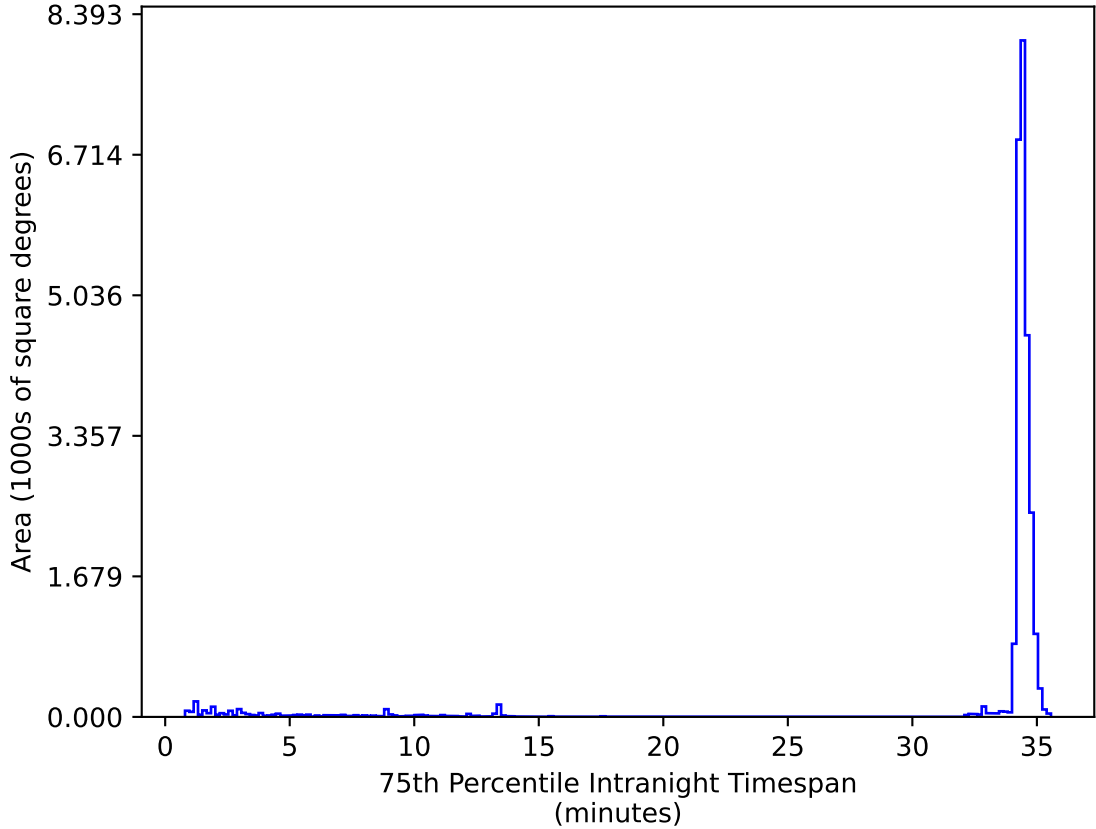
too_elab_heavy_r32_d3_griz_v3.4_10yrs All sky zy bands: 75th Percentile Intranight Timespan
