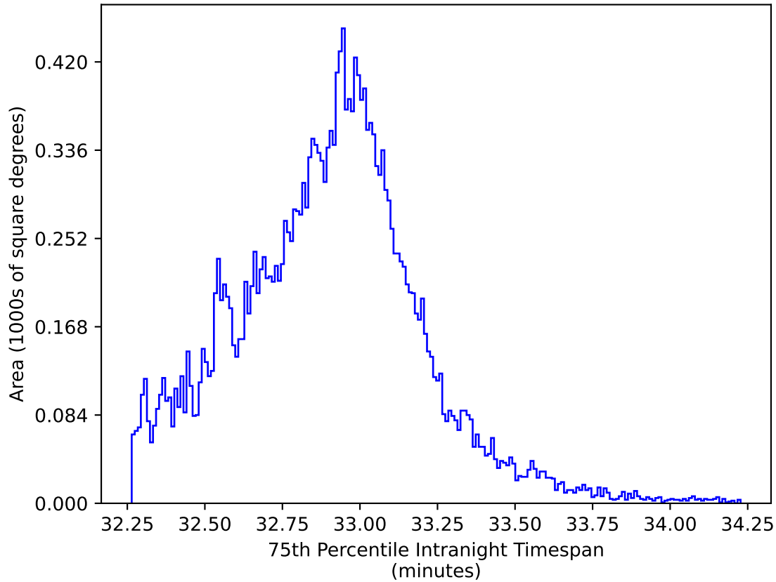
too_elab_heavy_r32_d3_griz_v3.4_10yrs All sky y band: 75th Percentile Intranight Timespan
