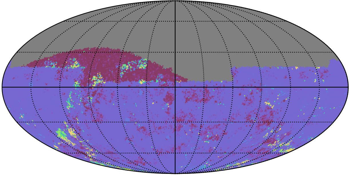
too_elab_heavy_r32_d3_griz_v3.4_10yrs All sky ug bands: 75th Percentile Intranight Timespan
