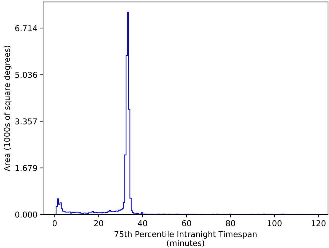
too_elab_heavy_r32_d3_griz_v3.4_10yrs All sky ug bands: 75th Percentile Intranight Timespan
