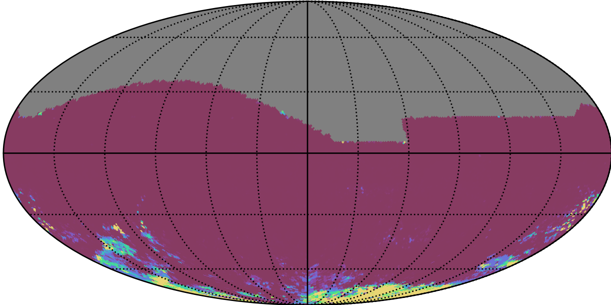
too_elab_heavy_r32_d3_griz_v3.4_10yrs All sky ri bands: 75th Percentile Intranight Timespan
