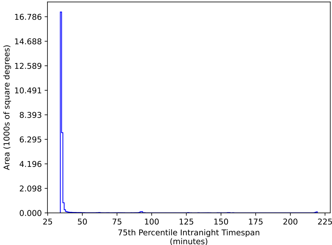
too_elab_heavy_r32_d3_griz_v3.4_10yrs All sky ri bands: 75th Percentile Intranight Timespan
