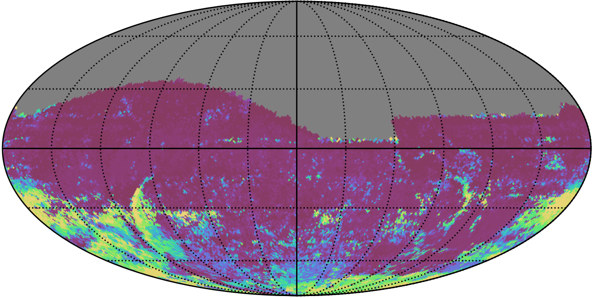
too_elab_heavy_r32_d3_griz_v3.4_10yrs All sky r band: 75th Percentile Intranight Timespan
