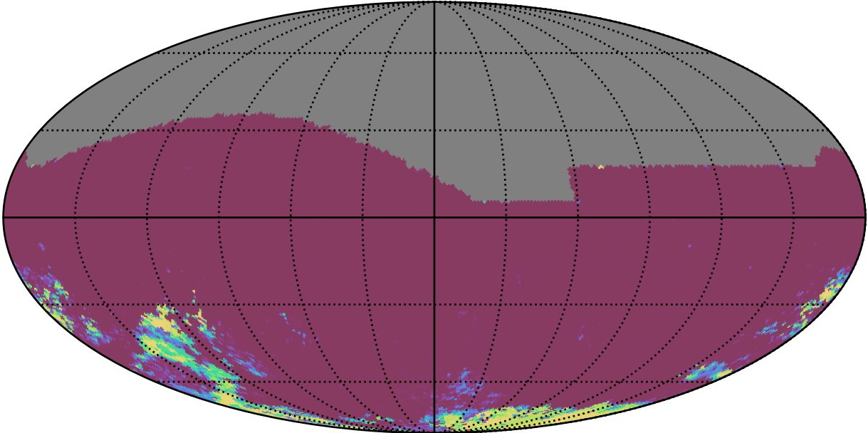
too_elab_heavy_r32_d3_griz_v3.4_10yrs All sky gr bands: 75th Percentile Intranight Timespan
