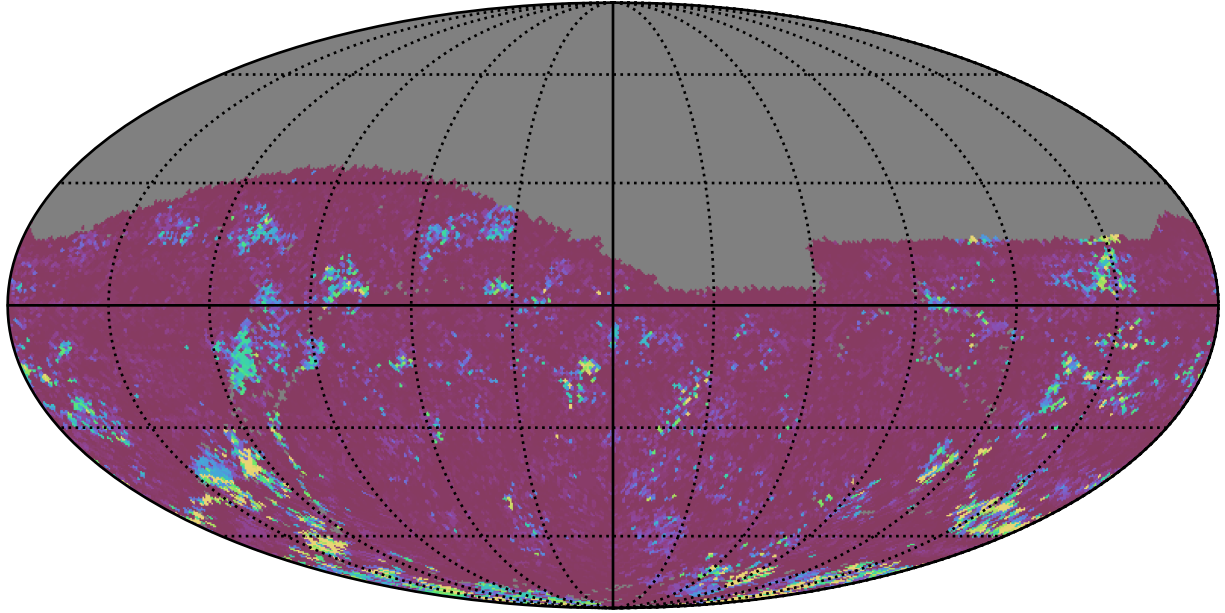
too_elab_heavy_r32_d3_griz_v3.4_10yrs All sky g band: 75th Percentile Intranight Timespan
