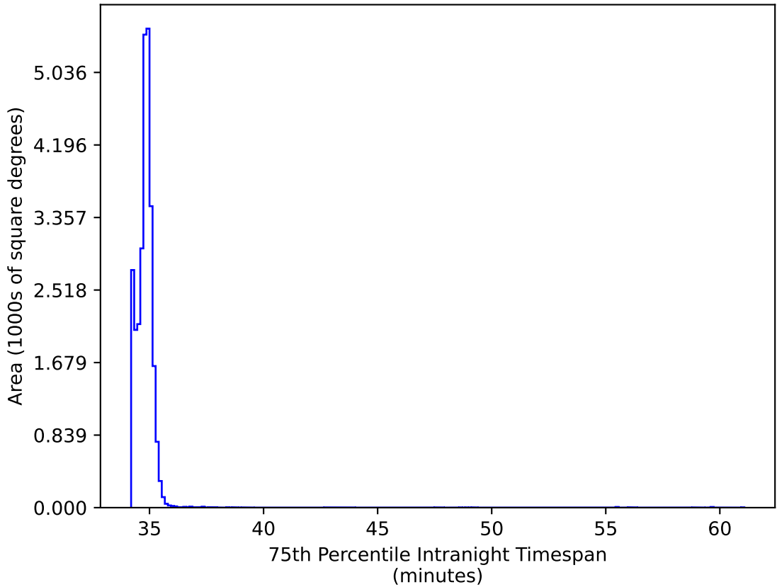
too_elab_heavy_r32_d3_griz_v3.4_10yrs All sky: 75th Percentile Intranight Timespan
