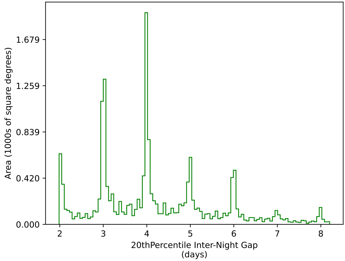
too_elab_heavy_r32_d3_griz_v3.4_10yrs WFD g band: 20thPercentile Inter-Night Gap
