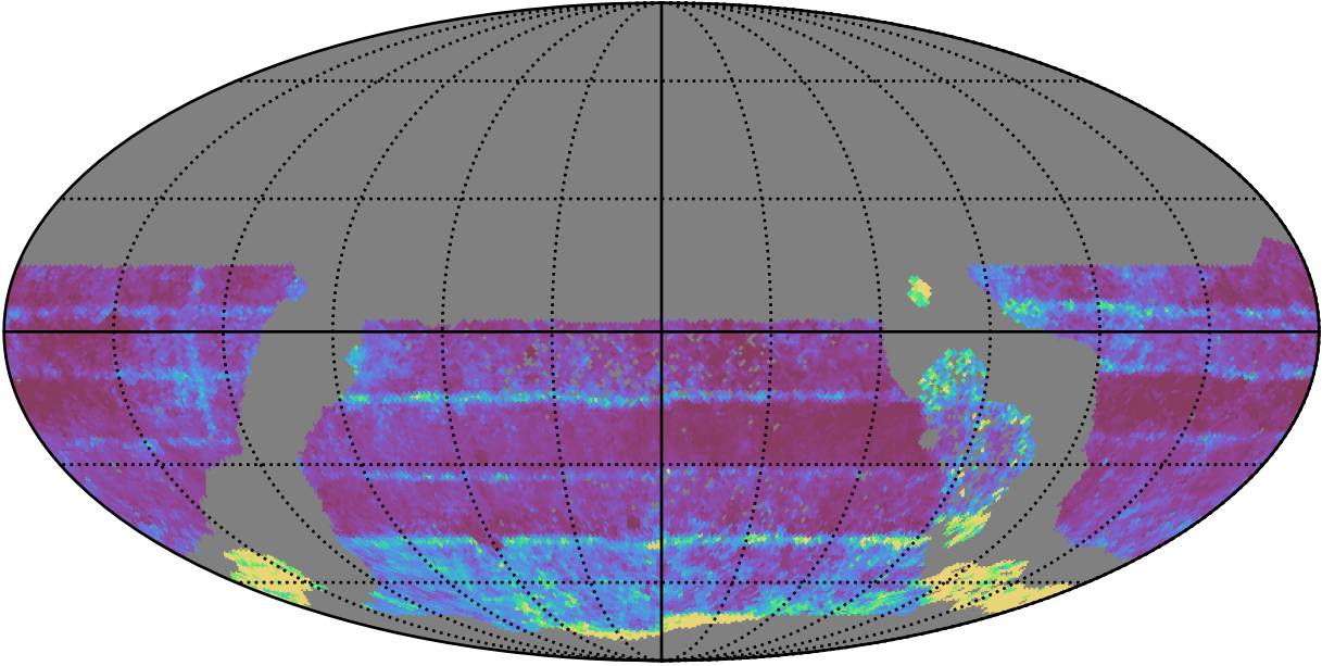
too_elab_heavy_r32_d3_griz_v3.4_10yrs WFD all bands: 20thPercentile Inter-Night Gap
