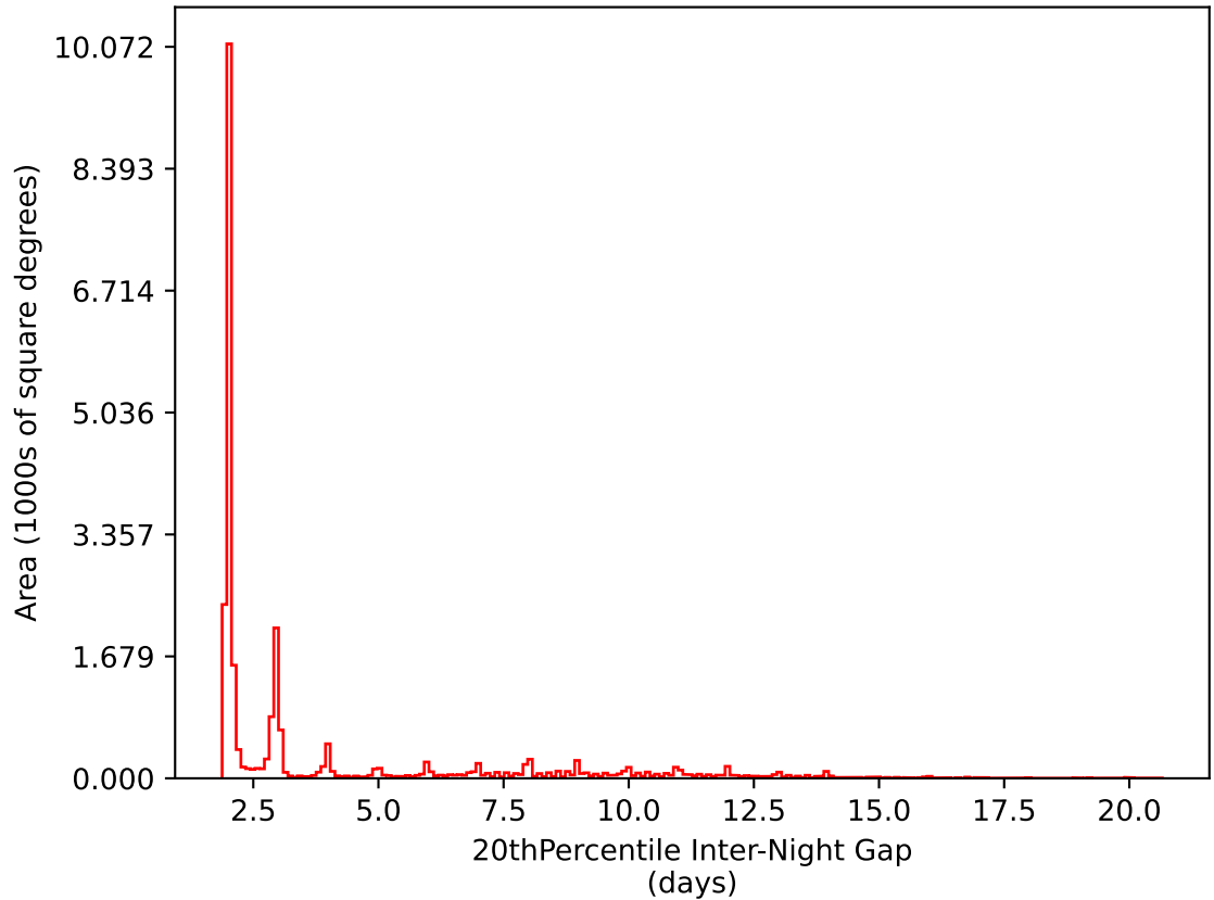
too_elab_heavy_r32_d3_griz_v3.4_10yrs All sky i band: 20thPercentile Inter-Night Gap
