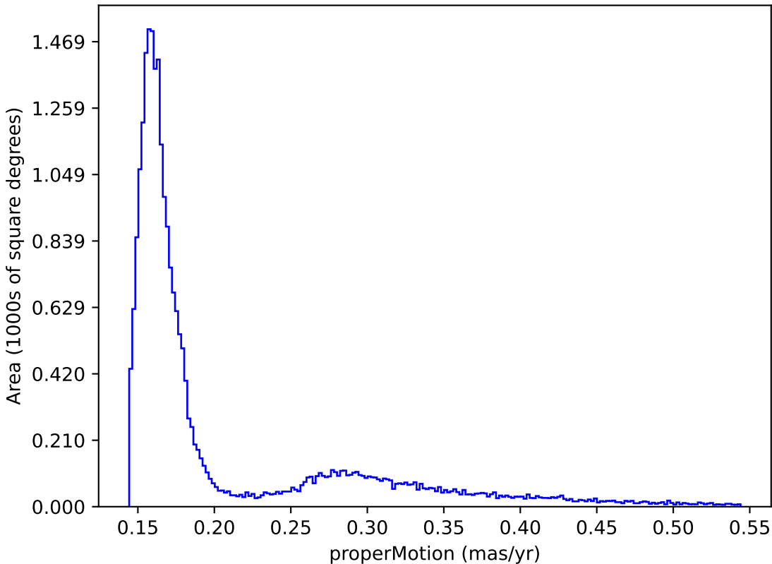
too_elab_heavy_r32_d3_griz_v3.4_10yrs : properMotion
