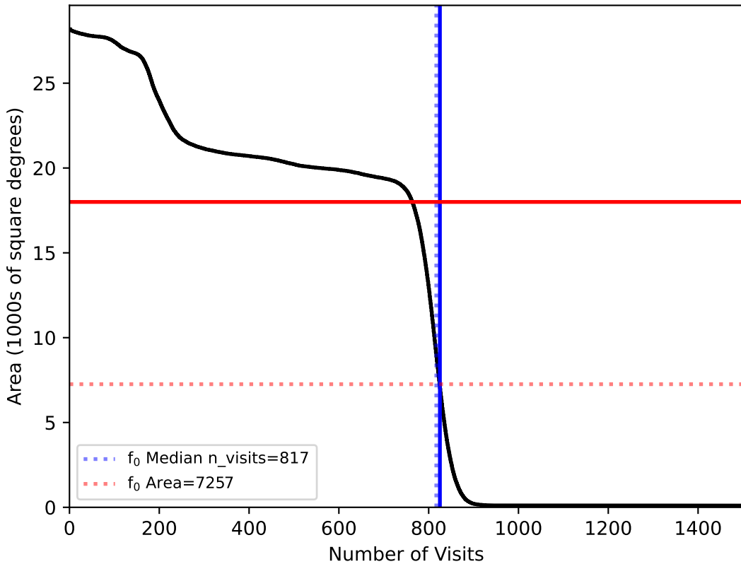
too_elab_heavy_r32_d3_griz_v3.4_10yrs : f0
