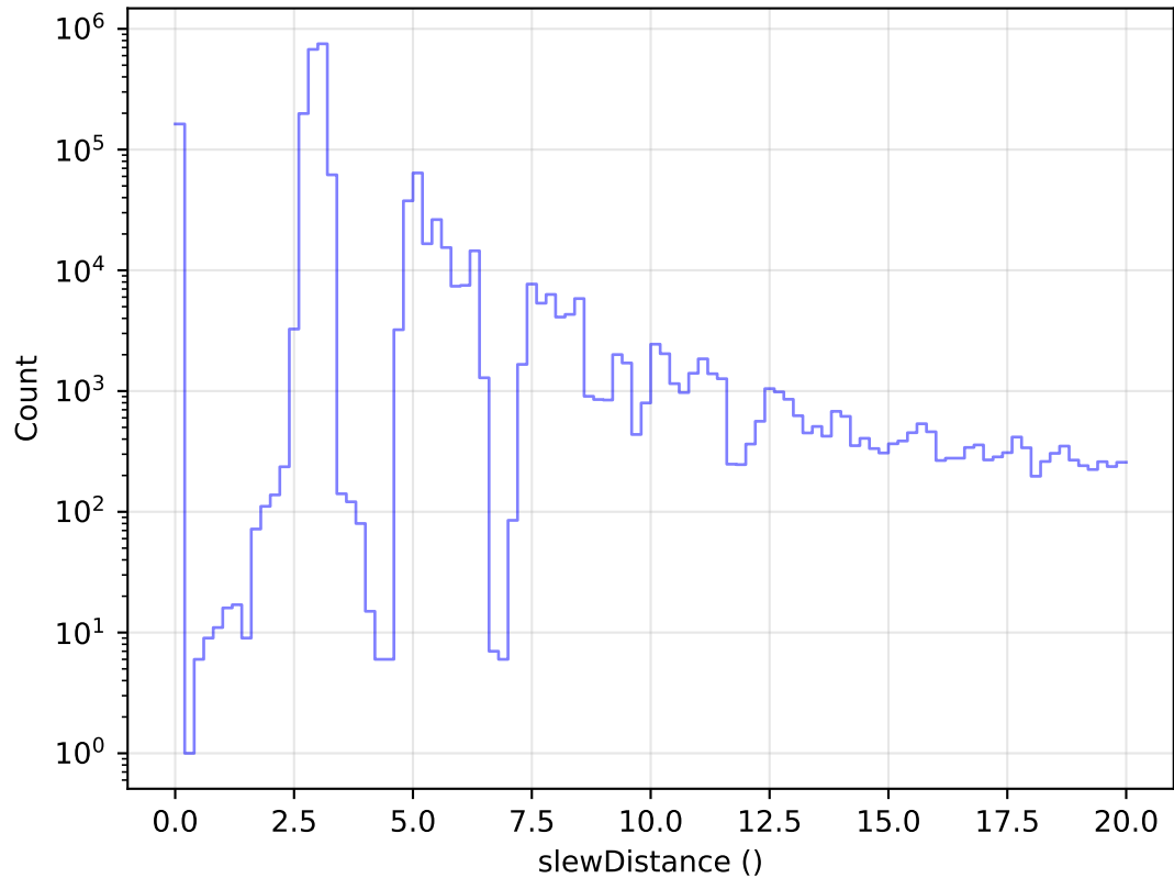
too_elab_heavy_r32_d3_griz_v3.4_10yrs All visits: Zoom Slew Distance Histogram
