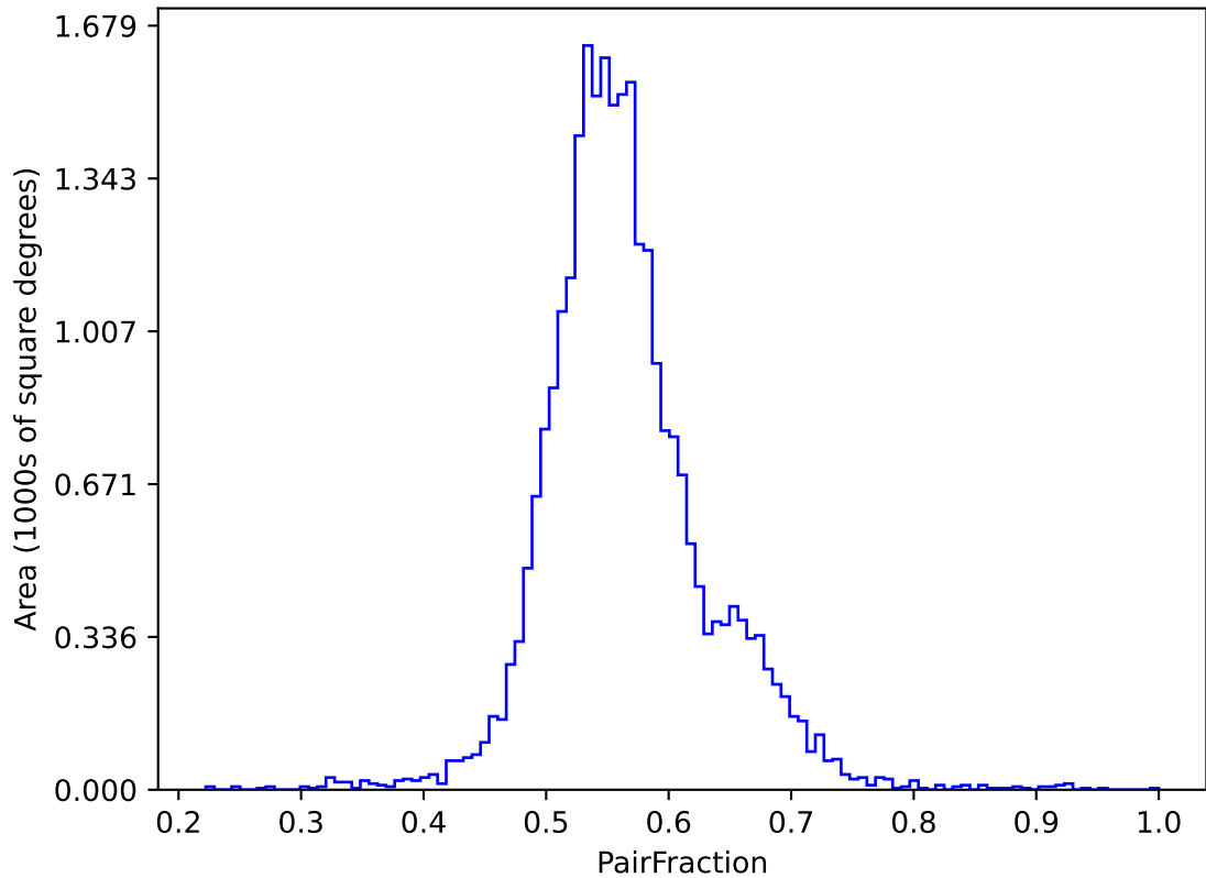
too_elab_heavy_r32_d3_griz_v3.4_10yrs (g or r or i): PairFraction
