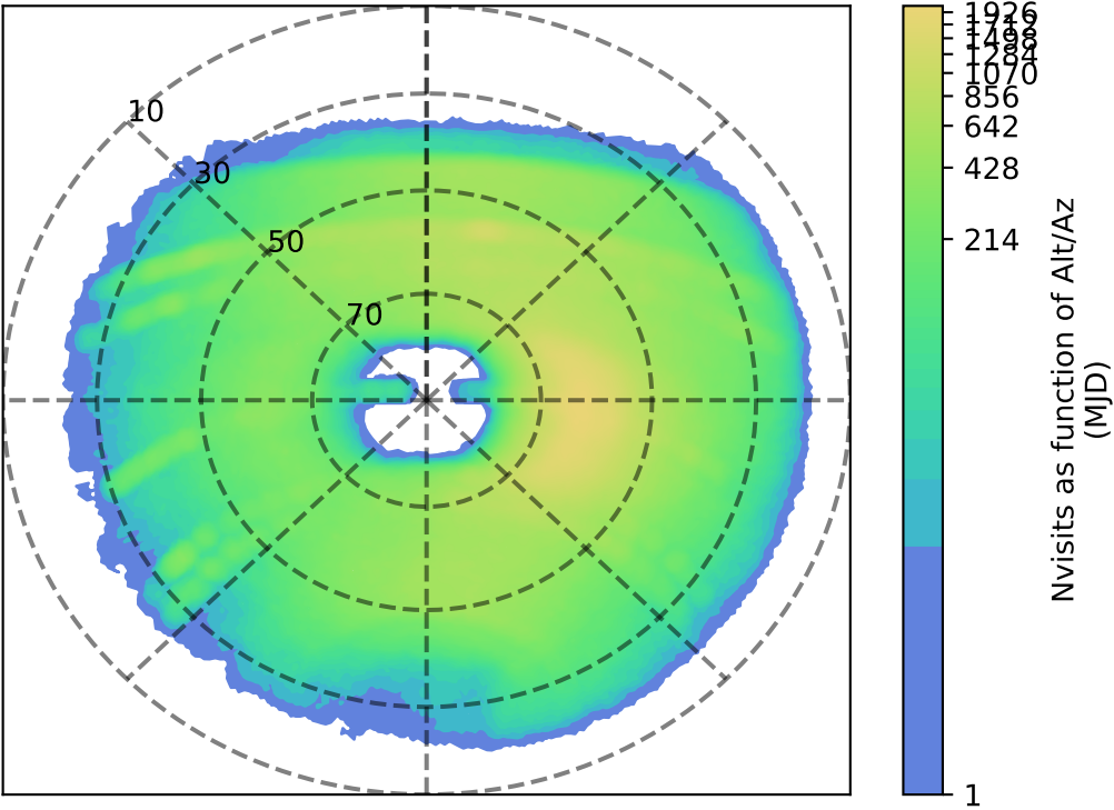
too_elab_heavy_r32_d3_griz_v3.4_10yrs y: Nvisits as function of Alt/Az
