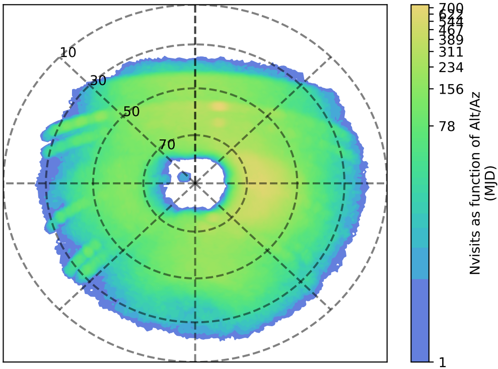
too_elab_heavy_r32_d3_griz_v3.4_10yrs u: Nvisits as function of Alt/Az
