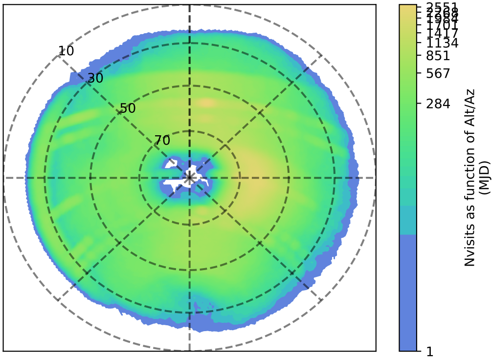
too_elab_heavy_r32_d3_griz_v3.4_10yrs r: Nvisits as function of Alt/Az
