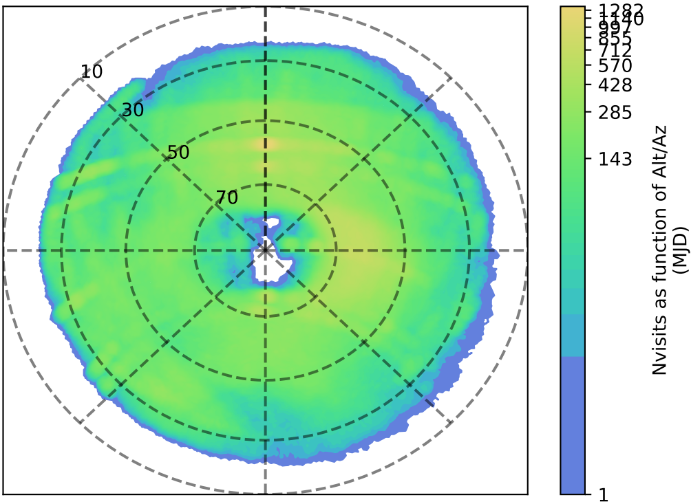
too_elab_heavy_r32_d3_griz_v3.4_10yrs g: Nvisits as function of Alt/Az
