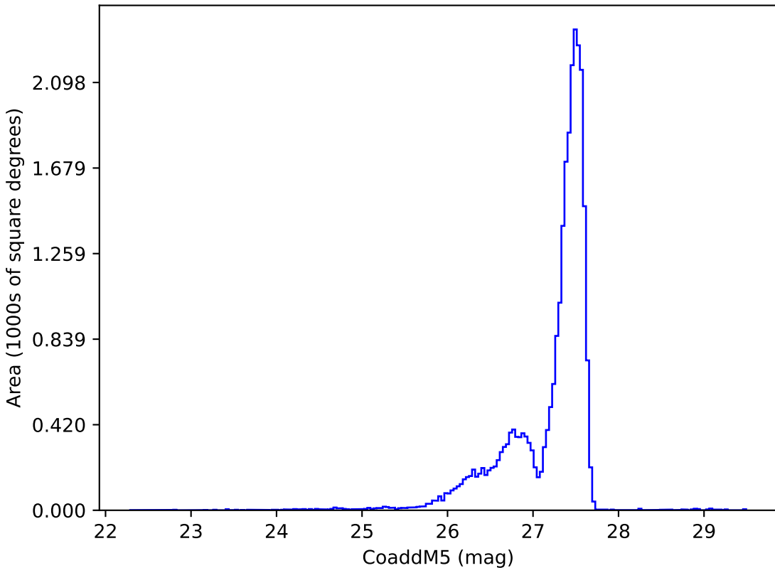
too_elab_heavy_r32_d3_griz_v3.4_10yrs : CoaddM5
