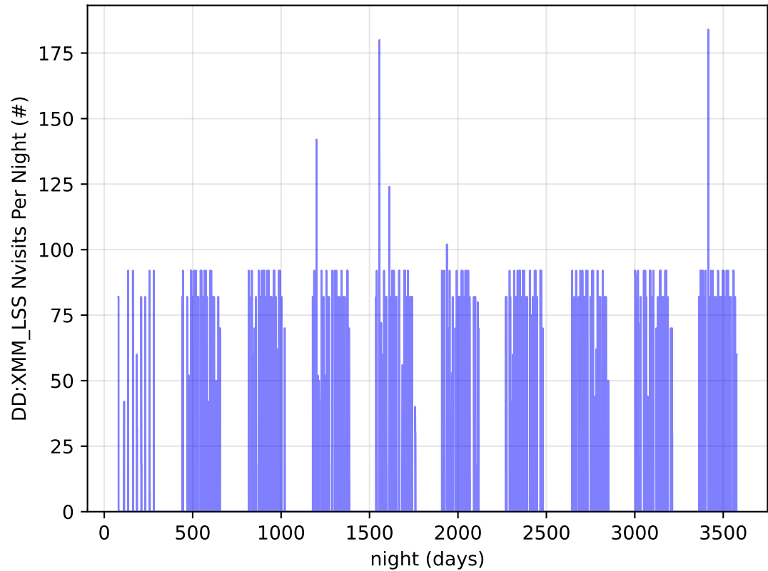
too_elab_heavy_r32_d3_griz_v3.4_10yrs all bands: DD:XMM_LSS Nvisits Per Night
