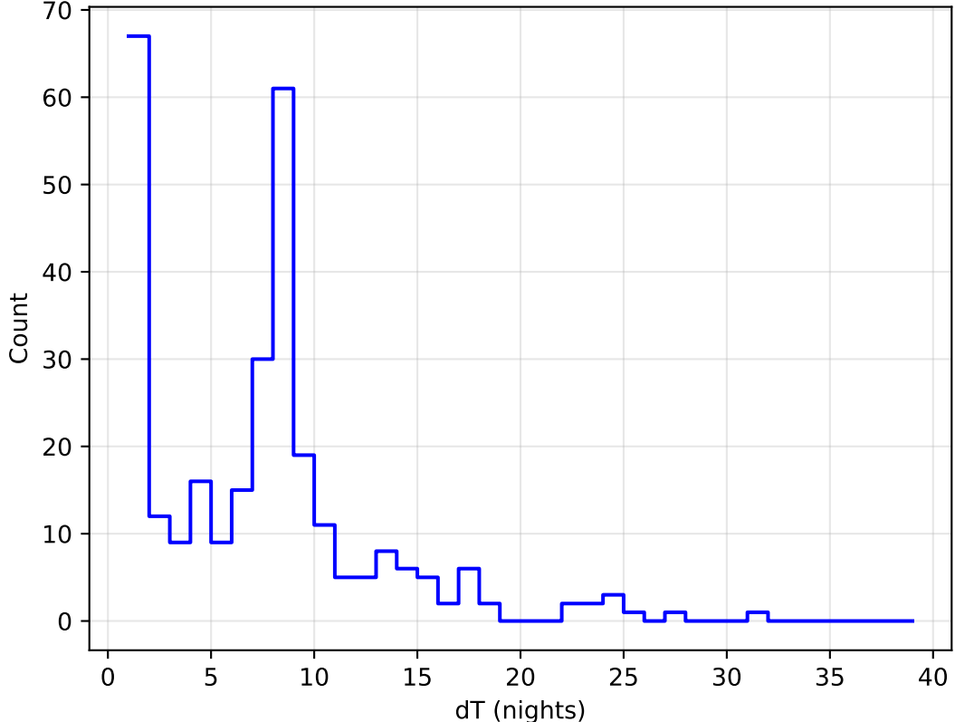
too_elab_heavy_r32_d3_griz_v3.4_10yrs all bands: DD:XMM_LSS Delta Nights Histogram
