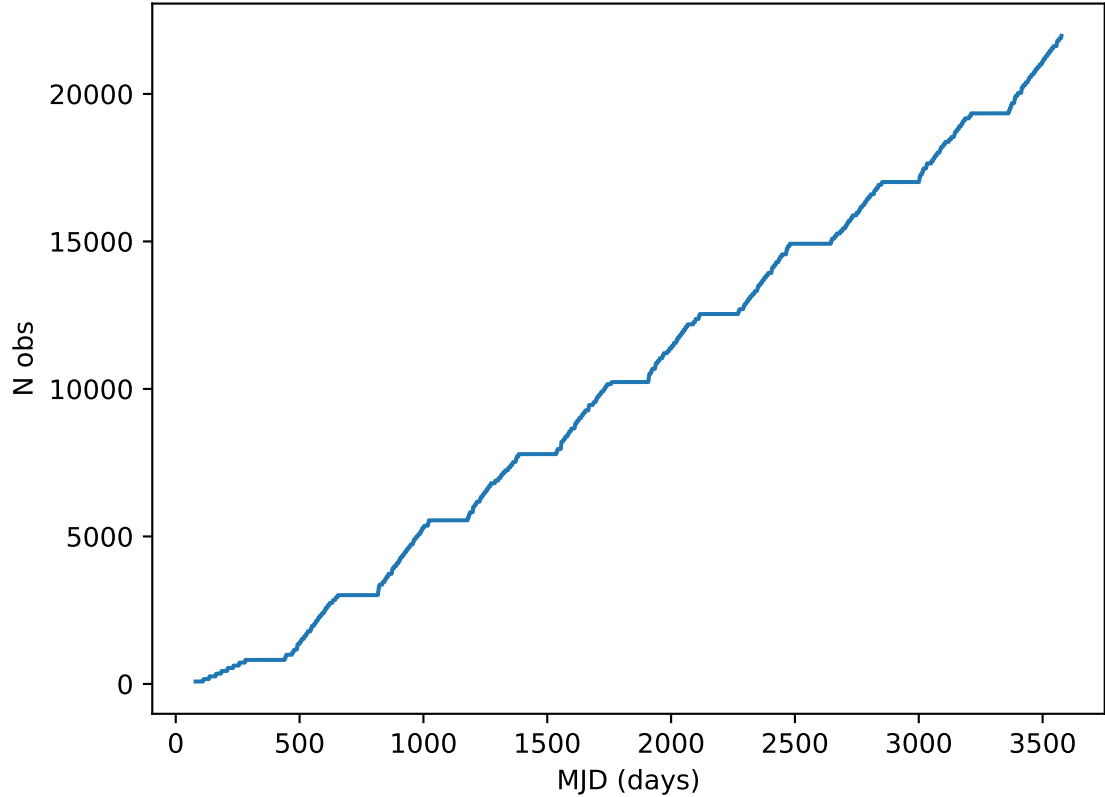
too_elab_heavy_r32_d3_griz_v3.4_10yrs all bands: DD:XMM_LSS Cumulative NVisits
