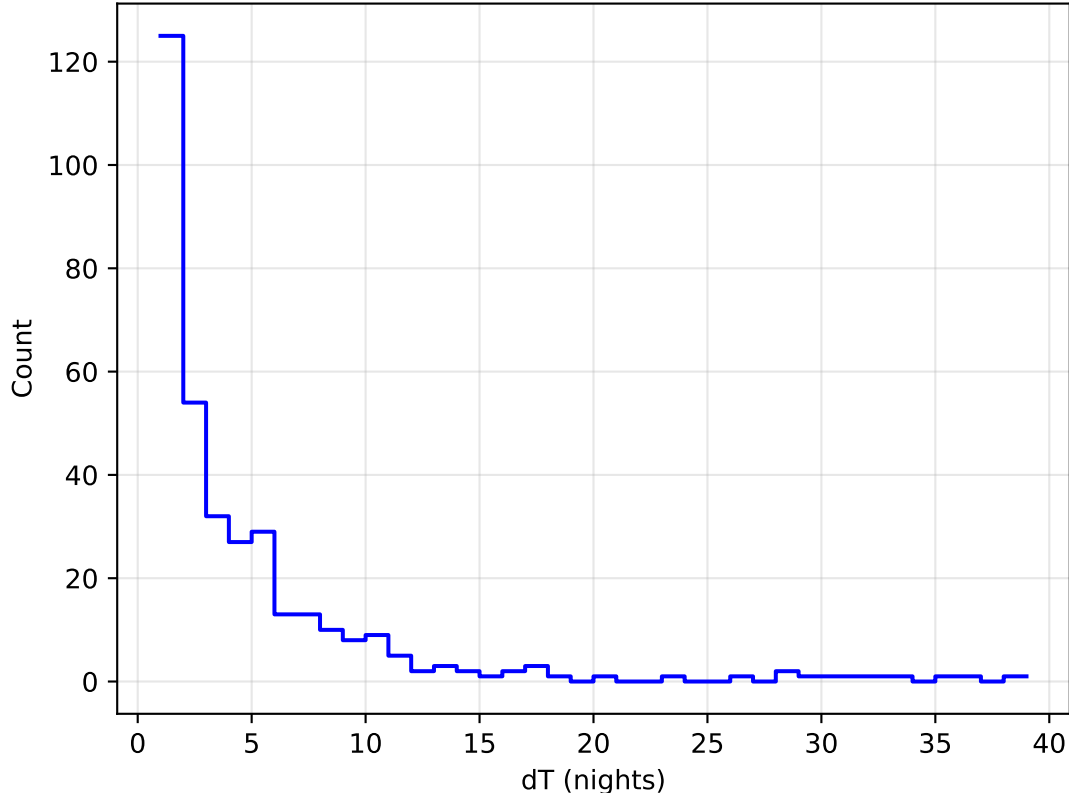
too_elab_heavy_r32_d3_griz_v3.4_10yrs all bands: DD:WFD Delta Nights Histogram
