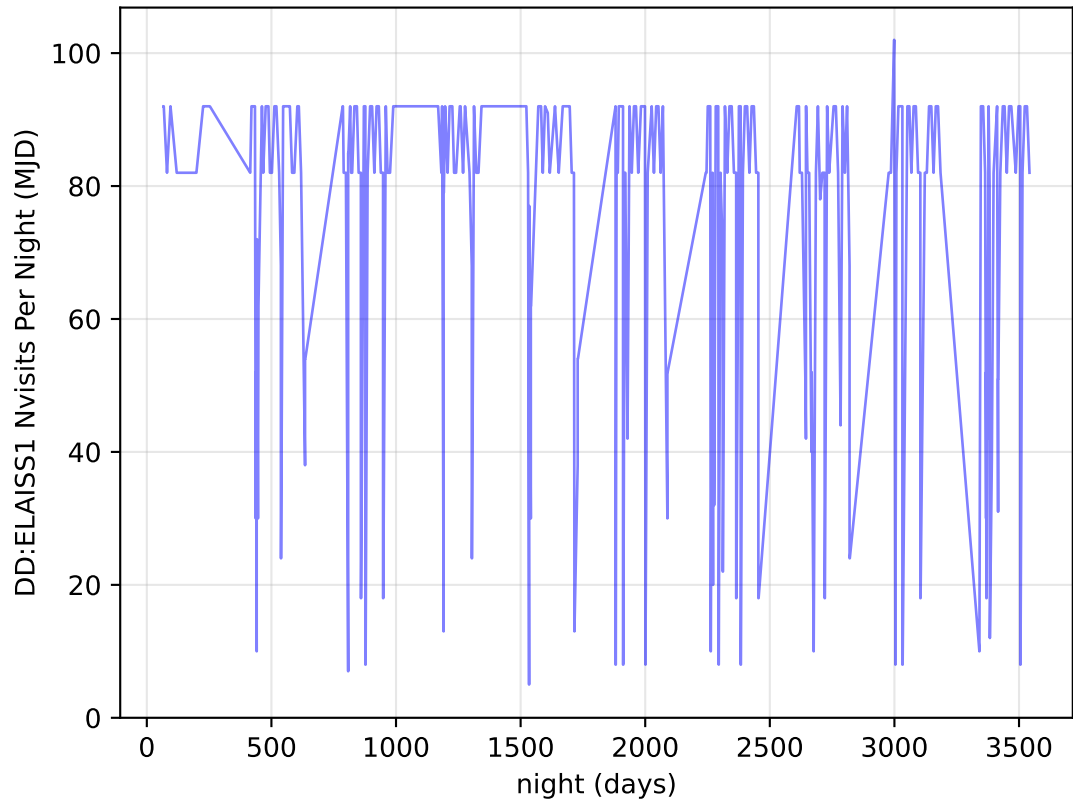
too_elab_heavy_r32_d3_griz_v3.4_10yrs all bands: DD:ELAISS1 Nvisits Per Night
