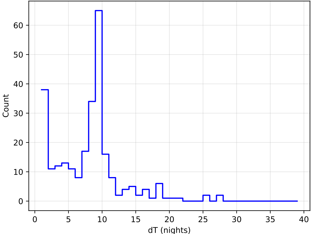
too_elab_heavy_r32_d3_griz_v3.4_10yrs all bands: DD:ELAISS1 Delta Nights Histogram
