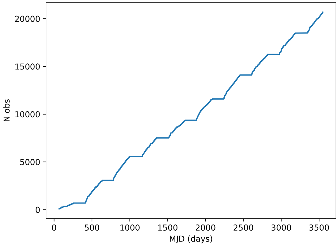
too_elab_heavy_r32_d3_griz_v3.4_10yrs all bands: DD:ELAISS1 Cumulative NVisits
