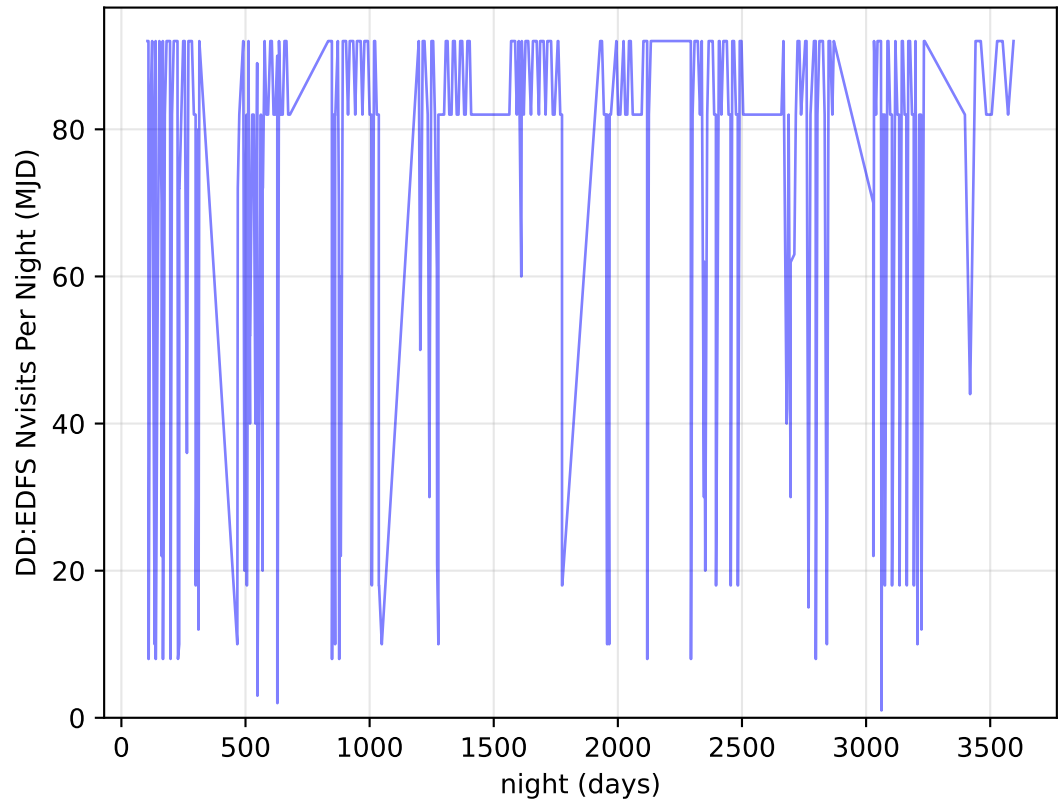
too_elab_heavy_r32_d3_griz_v3.4_10yrs all bands: DD:EDFS Nvisits Per Night
