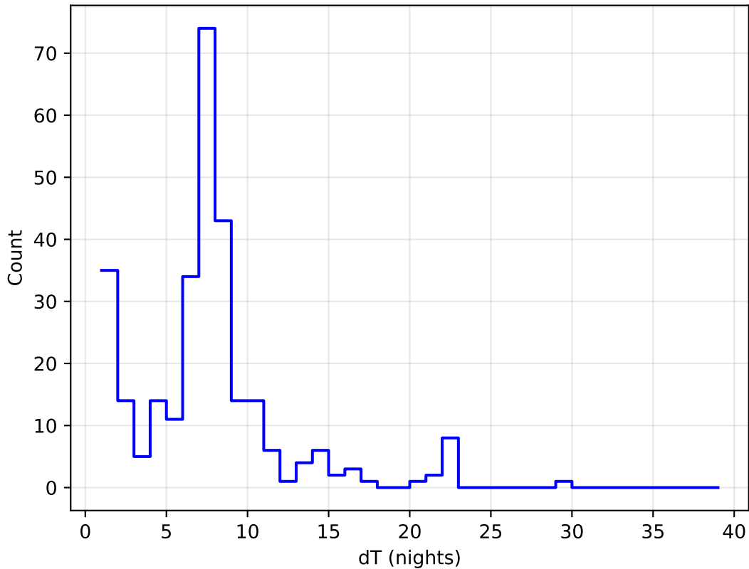
too_elab_heavy_r32_d3_griz_v3.4_10yrs all bands: DD:EDFS Delta Nights Histogram
