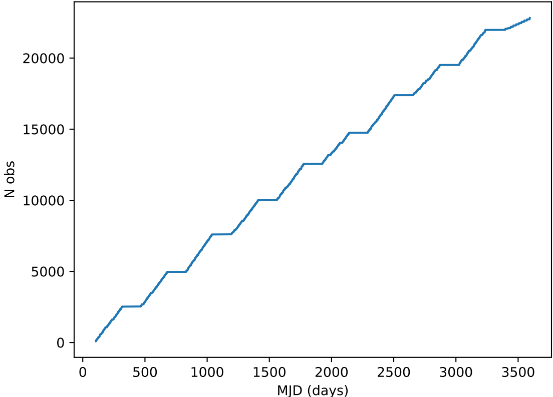
too_elab_heavy_r32_d3_griz_v3.4_10yrs all bands: DD:EDFS Cumulative NVisits
