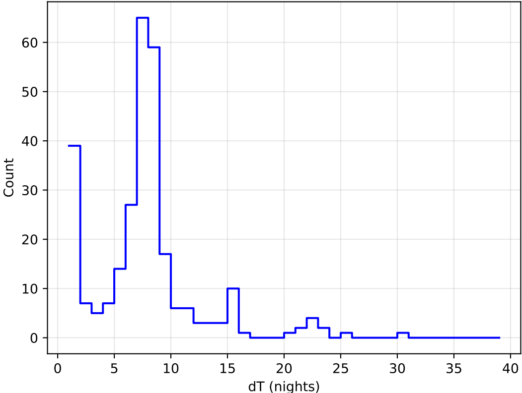
too_elab_heavy_r32_d3_griz_v3.4_10yrs all bands: DD:ECDFS Delta Nights Histogram
