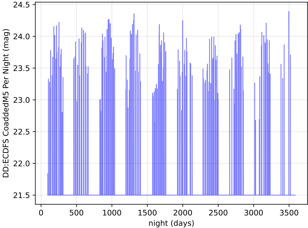
too_elab_heavy_r32_d3_griz_v3.4_10yrs y band: DD:ECDFS CoaddedM5 Per Night
