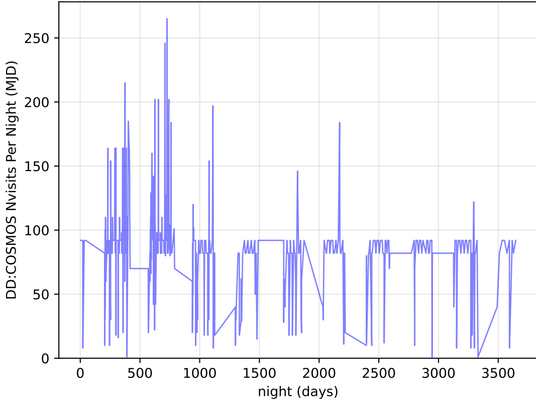
too_elab_heavy_r32_d3_griz_v3.4_10yrs all bands: DD: COSMOS Nvisits Per Night
