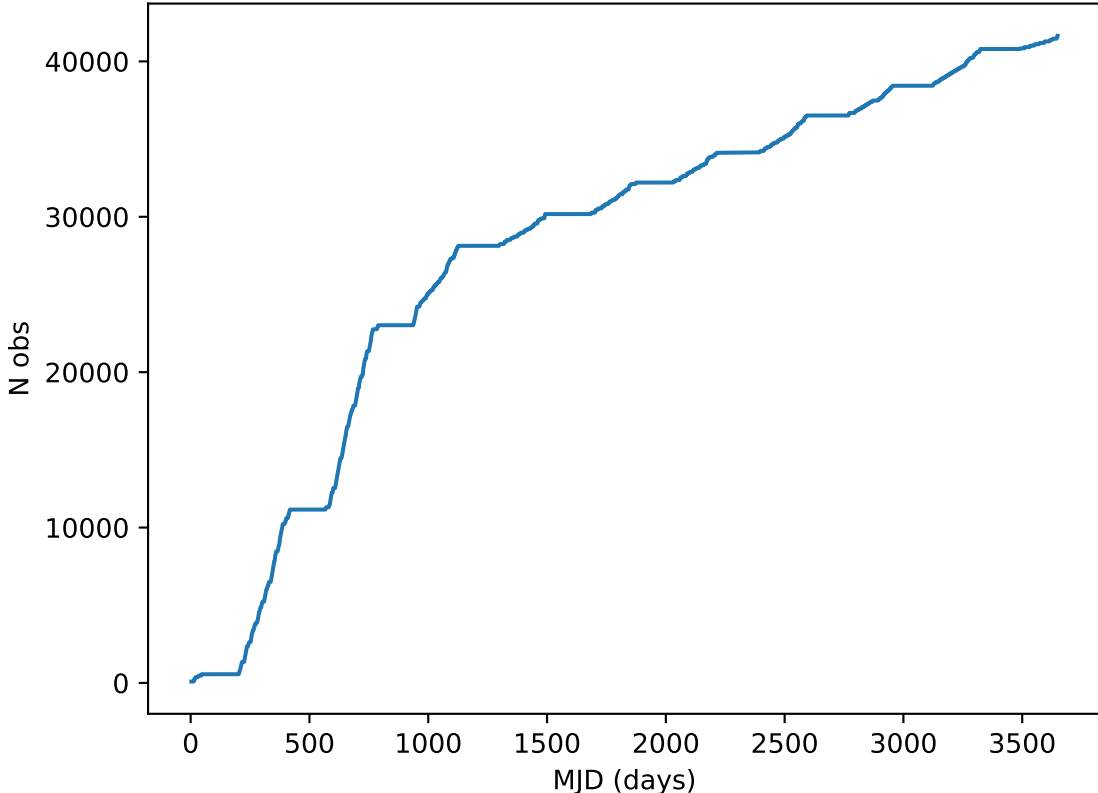
too_elab_heavy_r32_d3_griz_v3.4_10yrs all bands: DD: COSMOS Cumulative NVisits
