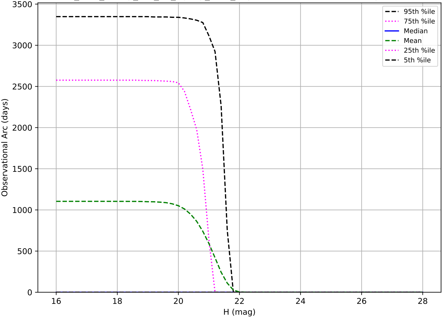
too_elab_heavy_r32_d2_ugrizy_v3.4_10yrs: Observational Arc Length Vatra
